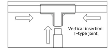
Intermediate Installation Method
