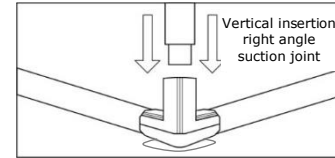
Installation method of four corner Foam tubes.
