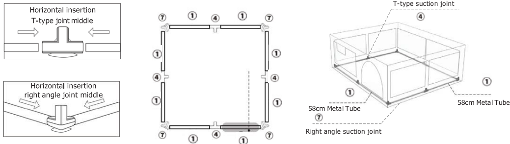
Bottom frame installation completion effect
